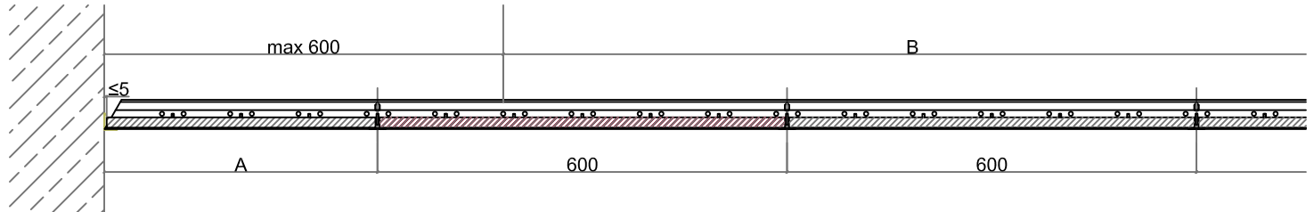
SUSPENDED CEILING ARRANGEMENT 1:20
