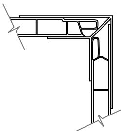
INTERNAL CORNER PROFILE 1:2
