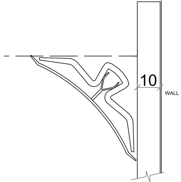
CEILING 2 PART COVE DETAIL 1:1
