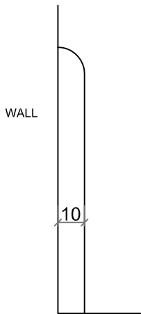
UPVC SKIRTING DETAIL 1:2
