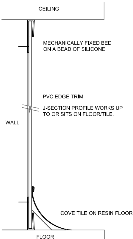
WALL TO FLOOR DETAIL 1:2
