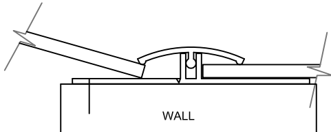
VERTICAL FIXING SINGLE 1:1
