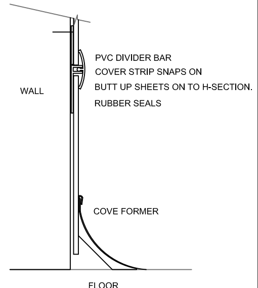
WALL TO FLOOR DETAIL 1:2
