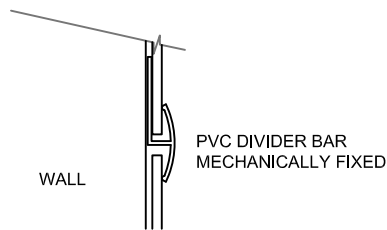
WALL TO FLOOR DETAIL 1:2
