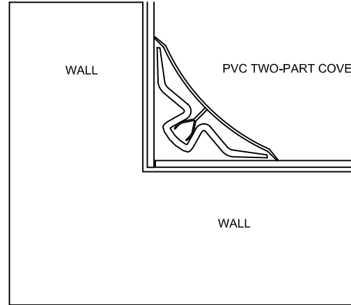
INTERNAL CORNER DETAIL 1:2
