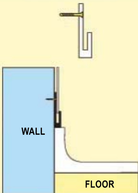
WALL TO FLOOR DETAIL
