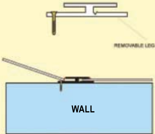
VERTICAL FIXING SINGLE
