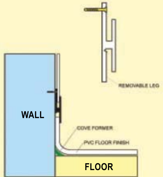
WALL TO FLOOR DETAIL
